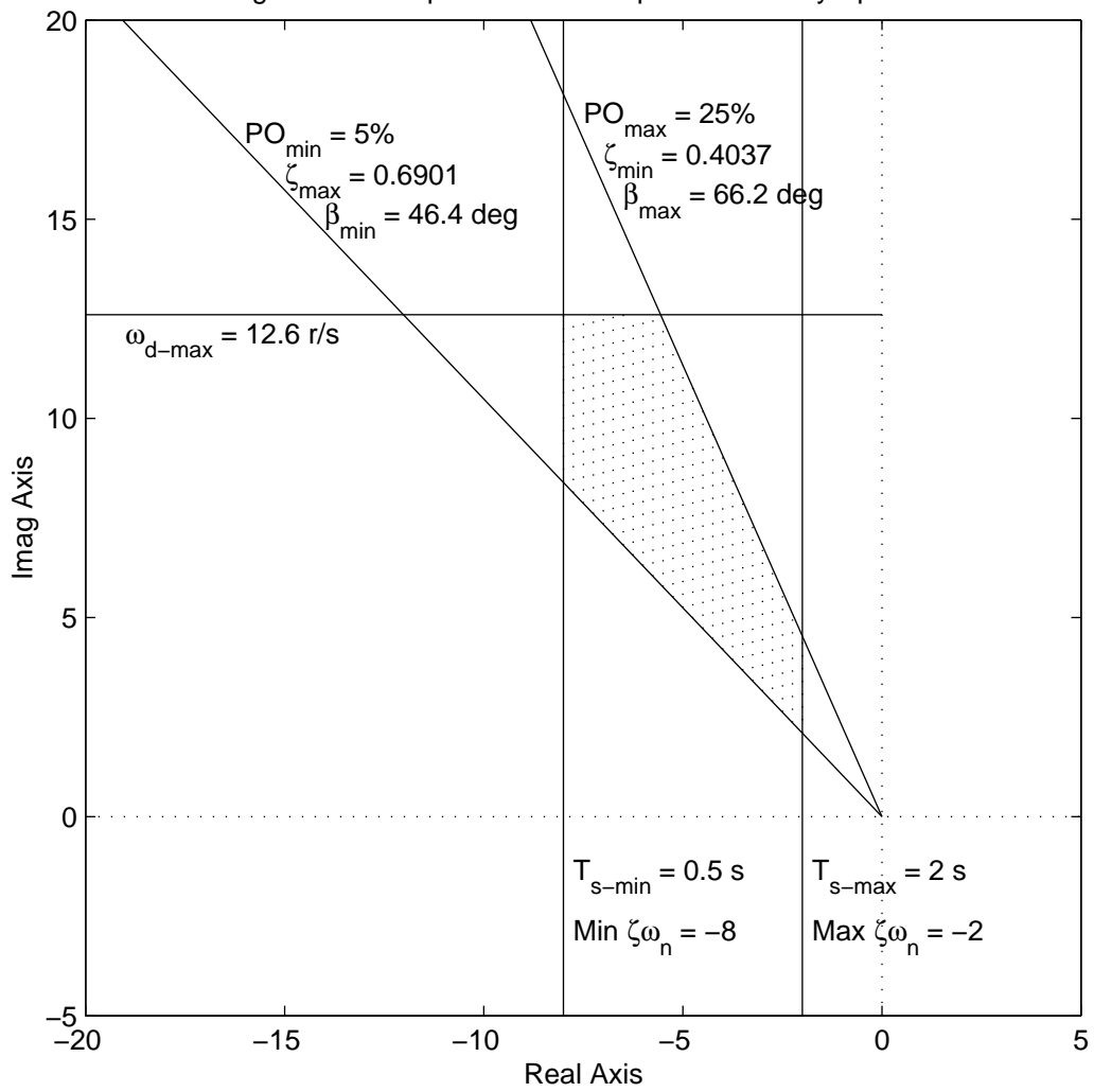
Locating Closed-Loop Poles in the s-plane to Satisfy Specifications
